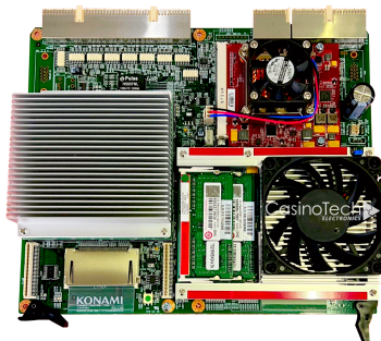
Konami KP3 CPU Board with Red Video Card
